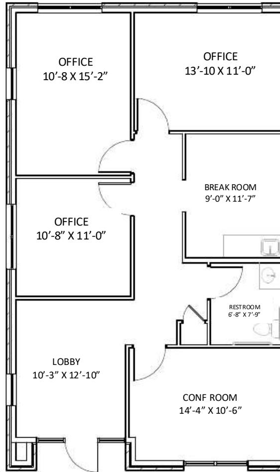
TYPICAL FLOOR PLAN – 1,187 SF SCALE 1/8" = 1'-0"
