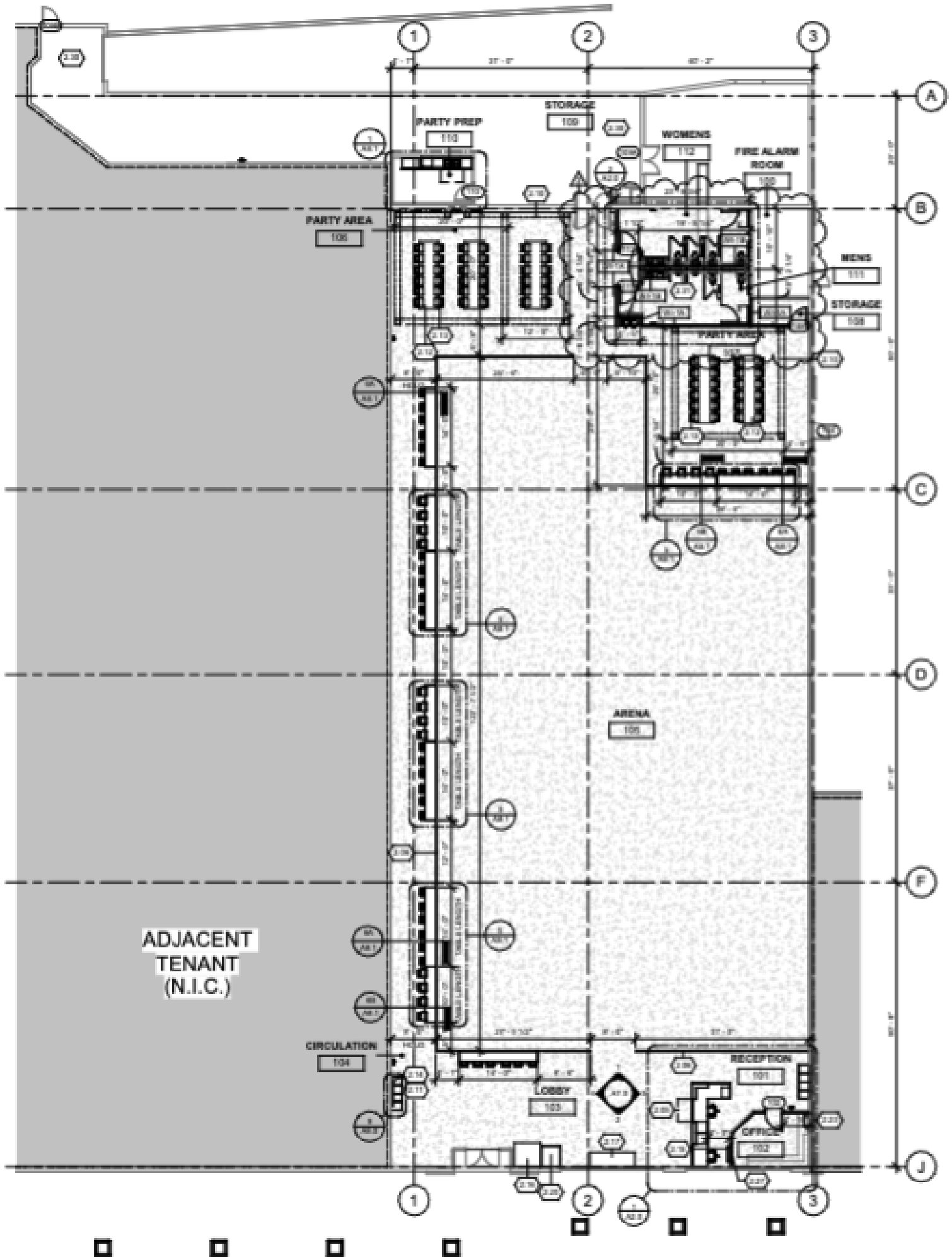
1 FLOOR PLAN 3/2" = 1'-0"
