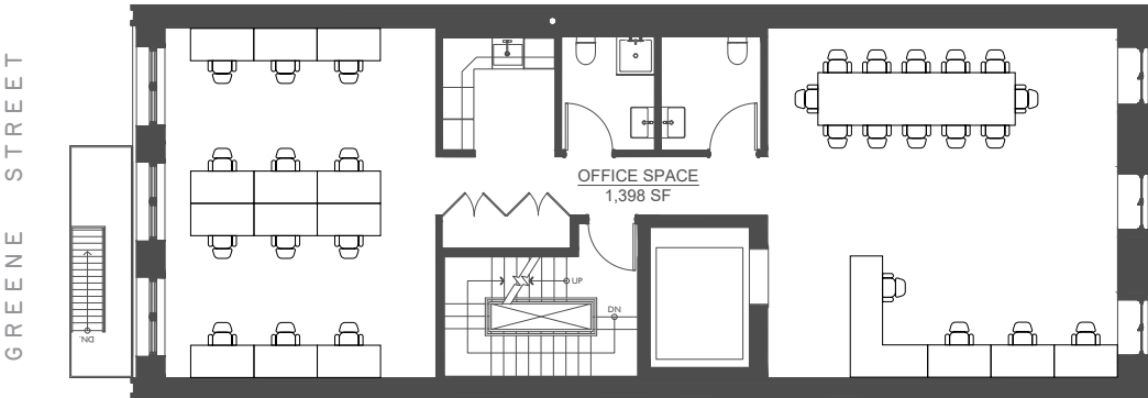
Third Floor
