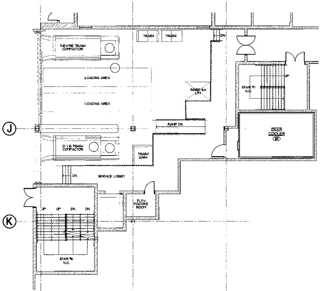
Second Floor Plan Layout
