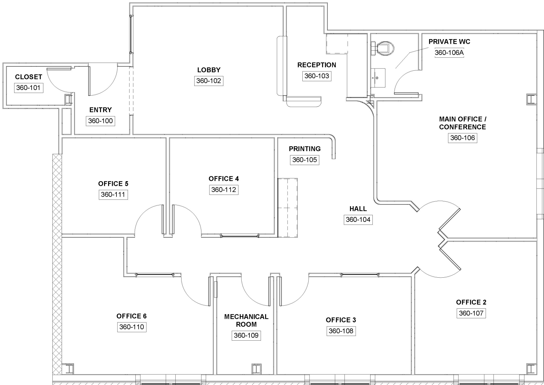
② Room Plan 1/4" = 1'-0"
