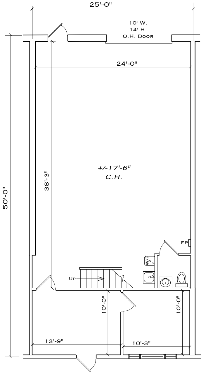
FIRST FLOOR 1,250 SQ. FT.
