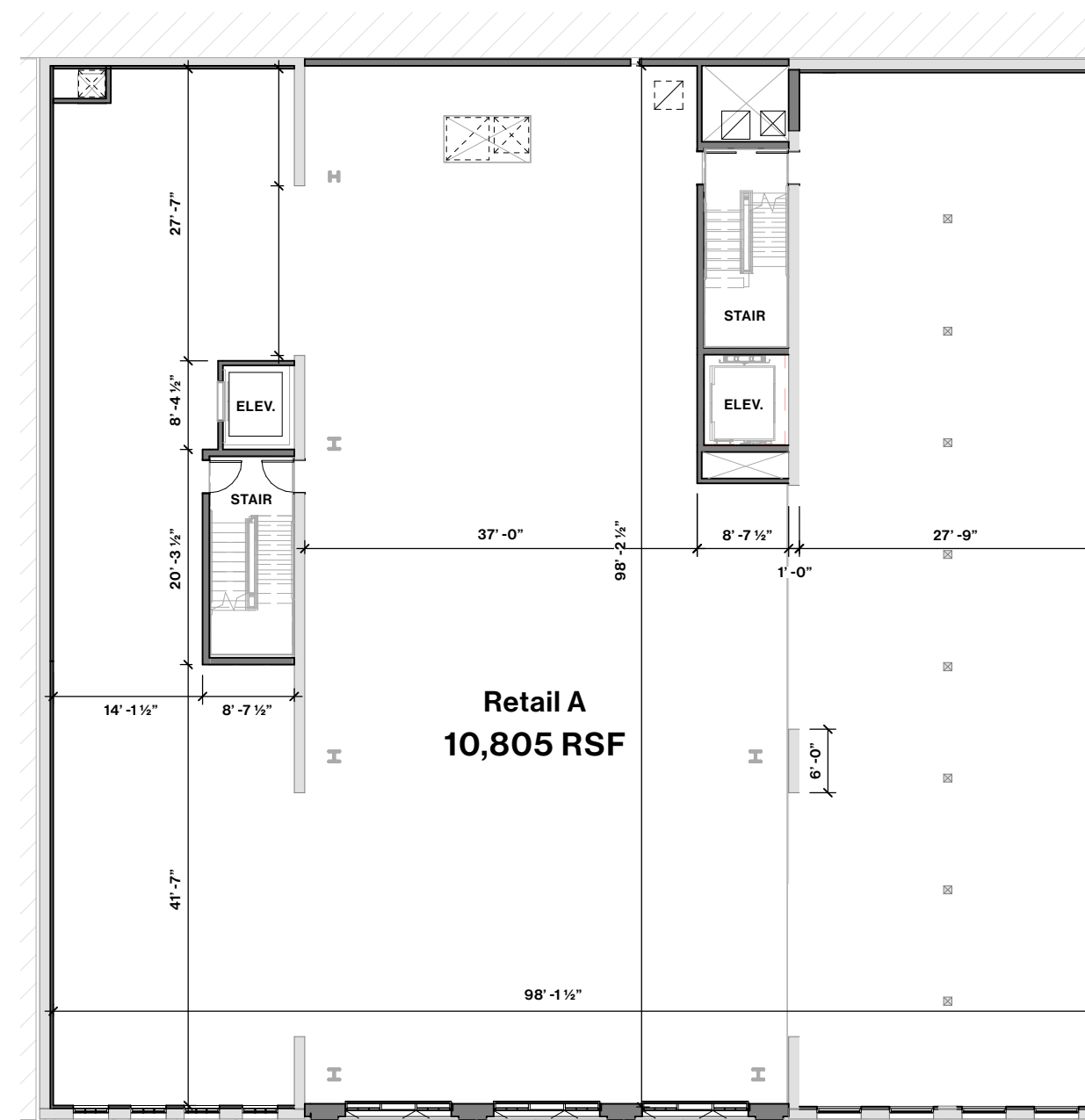
SECOND FLOOR — ±10,805 SF
