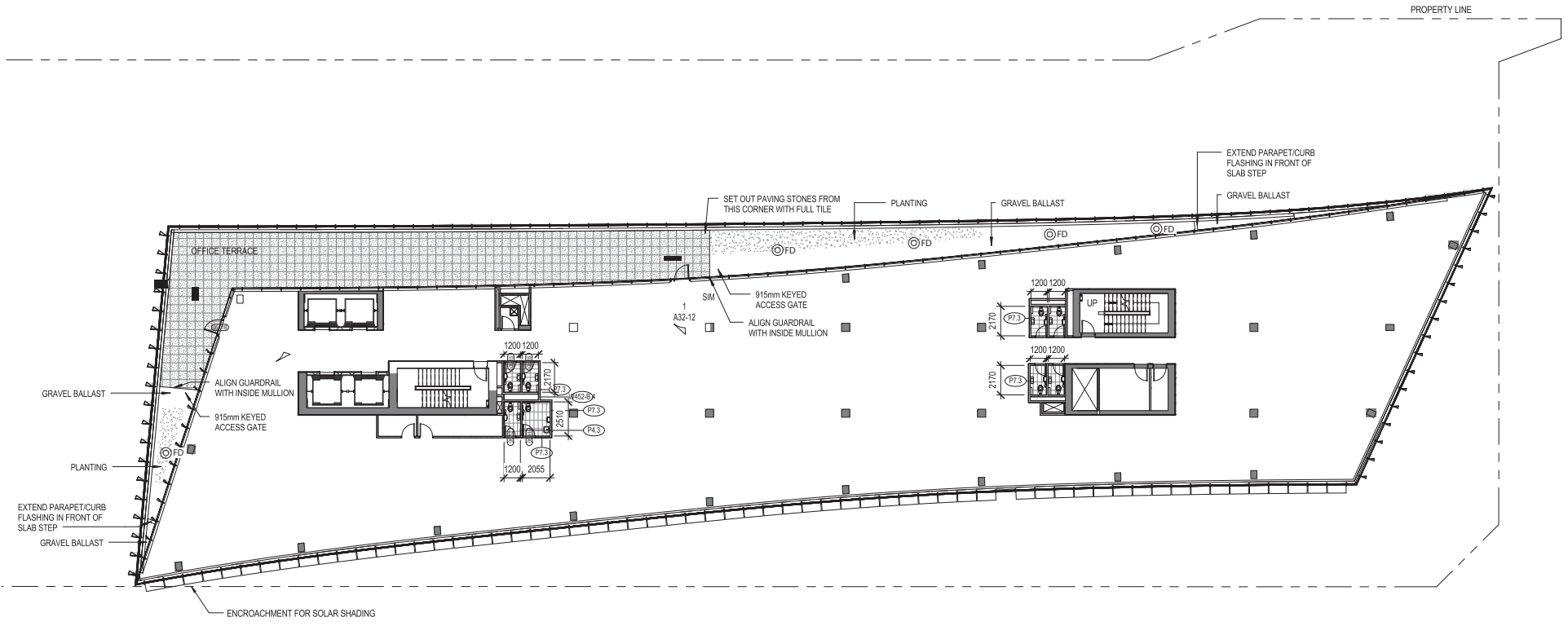
LEVEL 06 FLOOR PLAN
