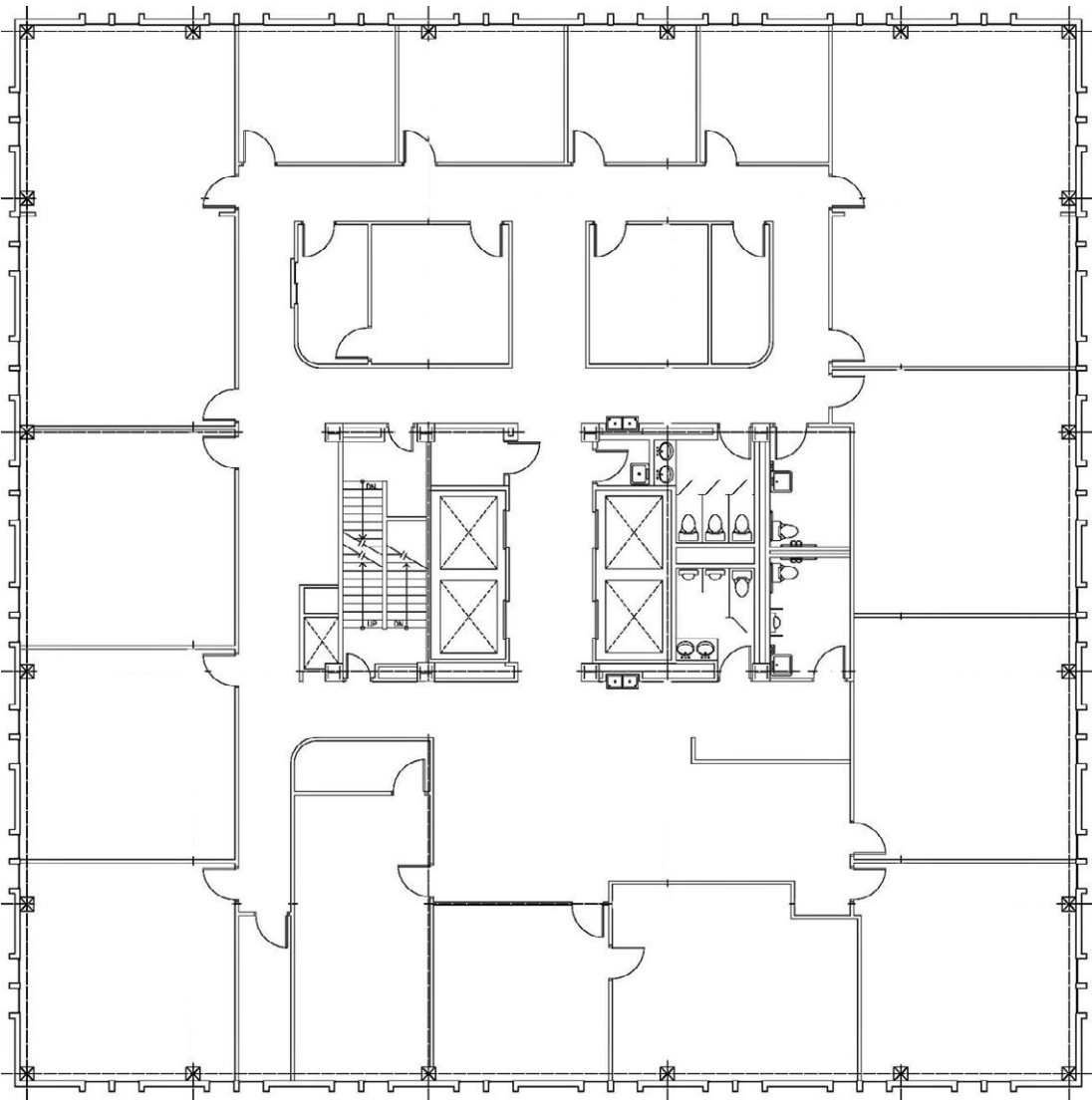
12TH FLOOR
