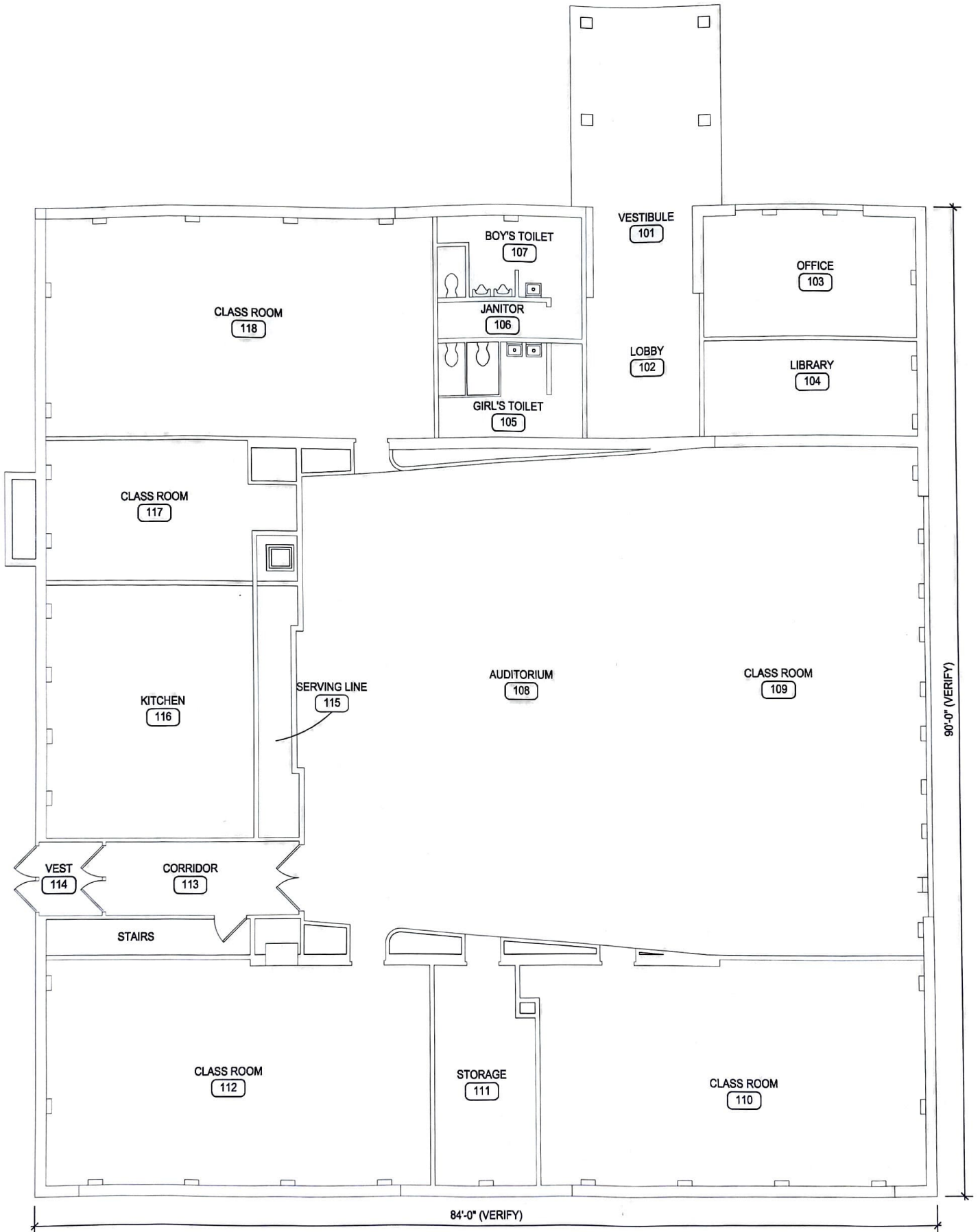
2 FIRST FLOOR PLAN A130 SCALE: 1/8" = 1'-0"
