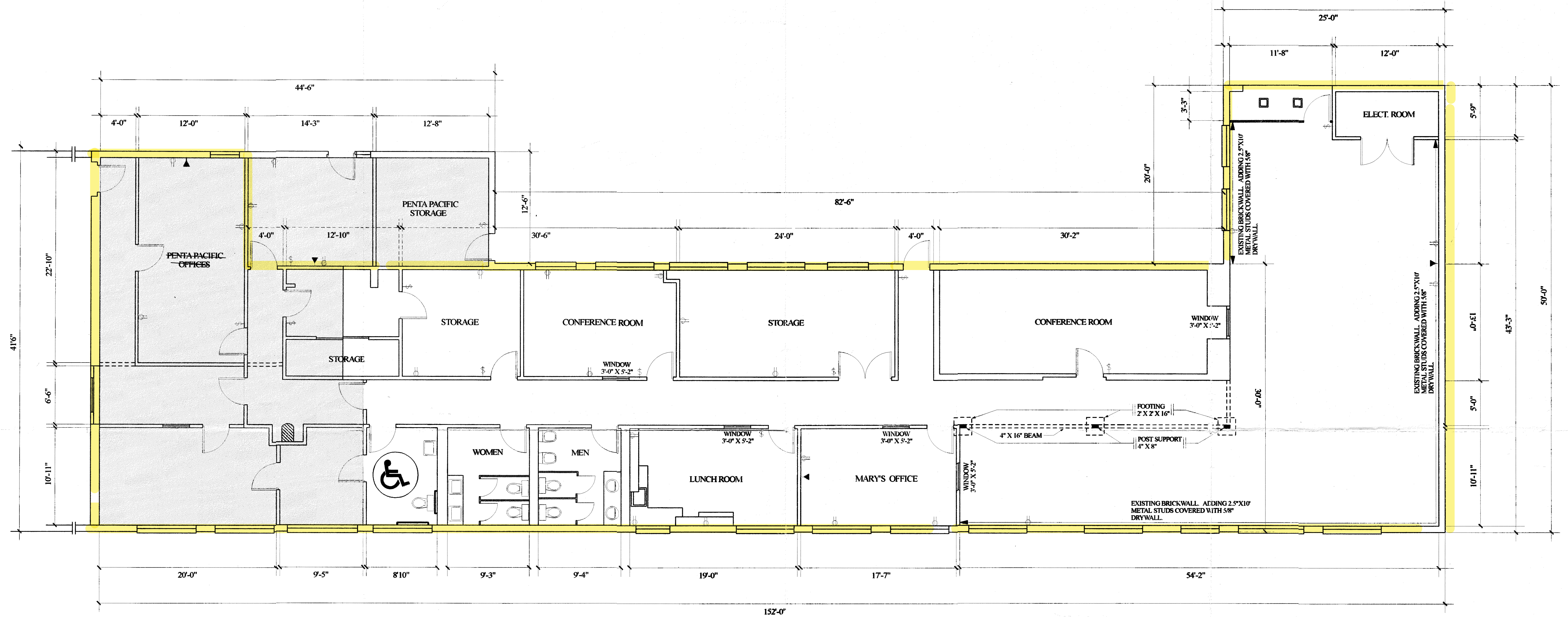
EXISTING OFFICE PLAN SCALE 1/8" = 1' - 0"
