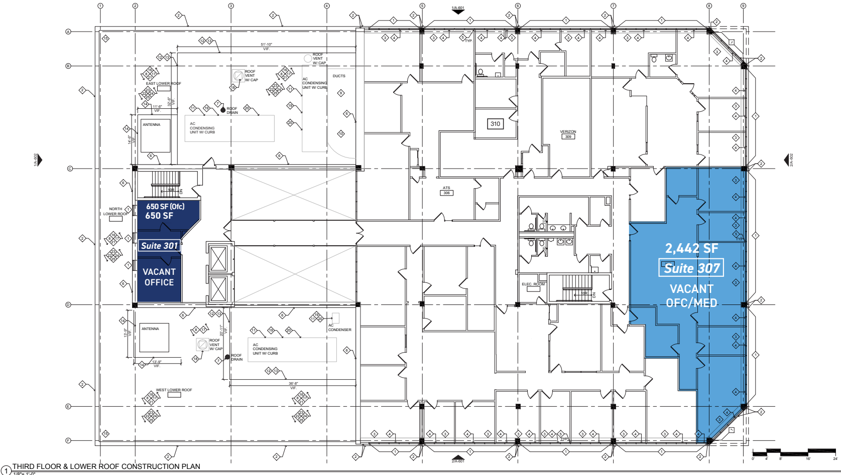
1 THIRD FLOOR & LOWER ROOF CONSTRUCTION PLAN 1/8" = 1'-0"
