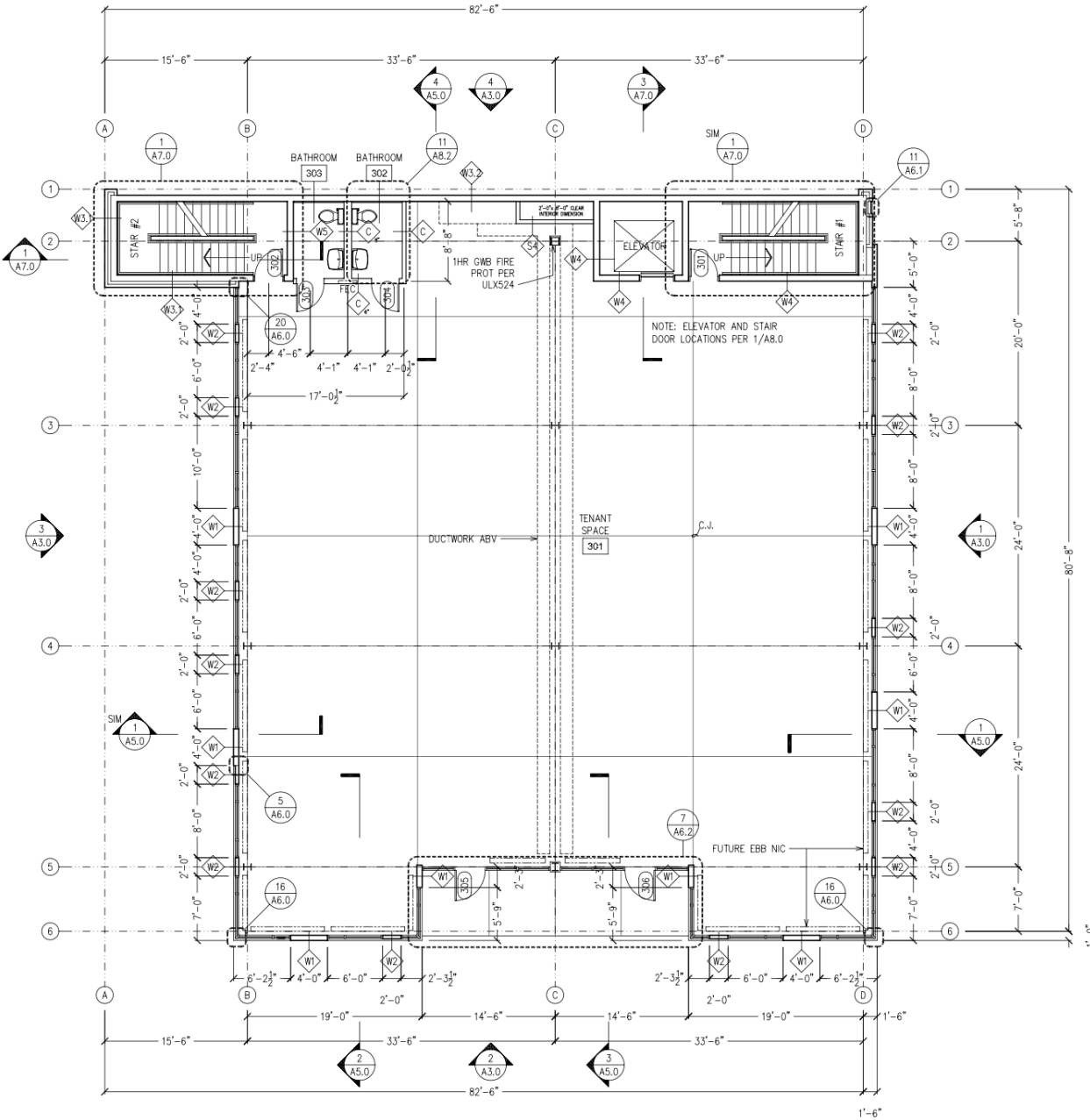
2 THIRD FLOOR PLAN SCALE: 1/8" = 1'-0" 0 4 8 16
