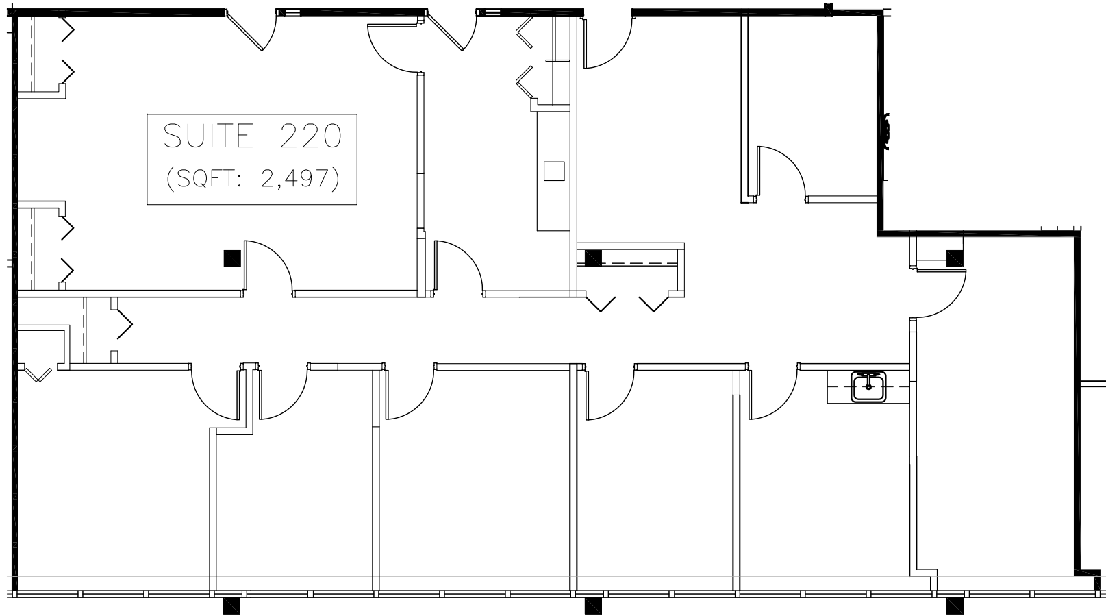
SUITE 220 - FLOOR PLAN sc: 1/8" = 1'-0"
