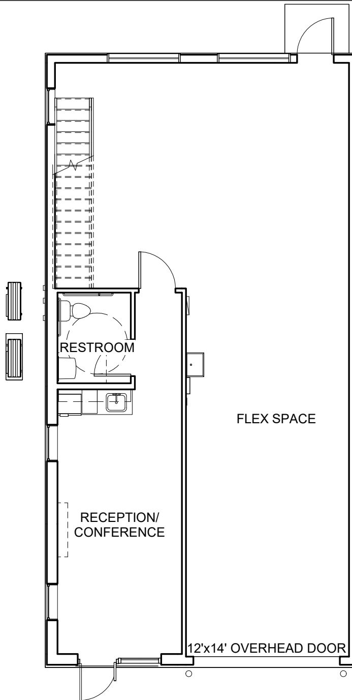
① Main Floor Marketing - 100C 1/8" = 1'-0"
