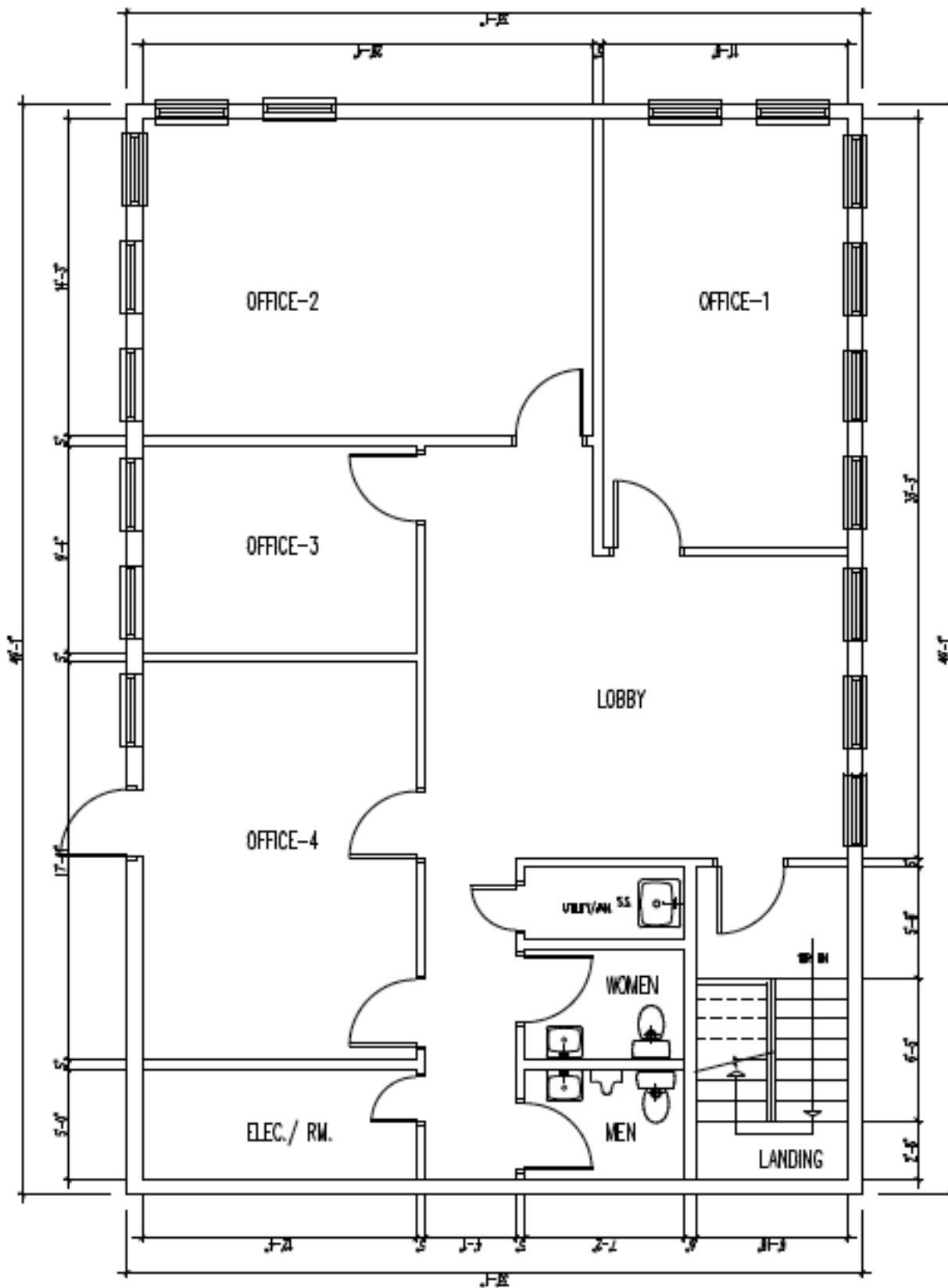
1 A-1 UPPER LEVEL PLAN SUITE - A SCALE: 1/4" = 1'-0"
