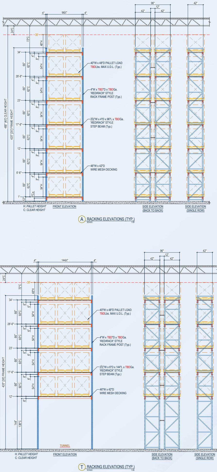
RACKING ELEVATIONS
