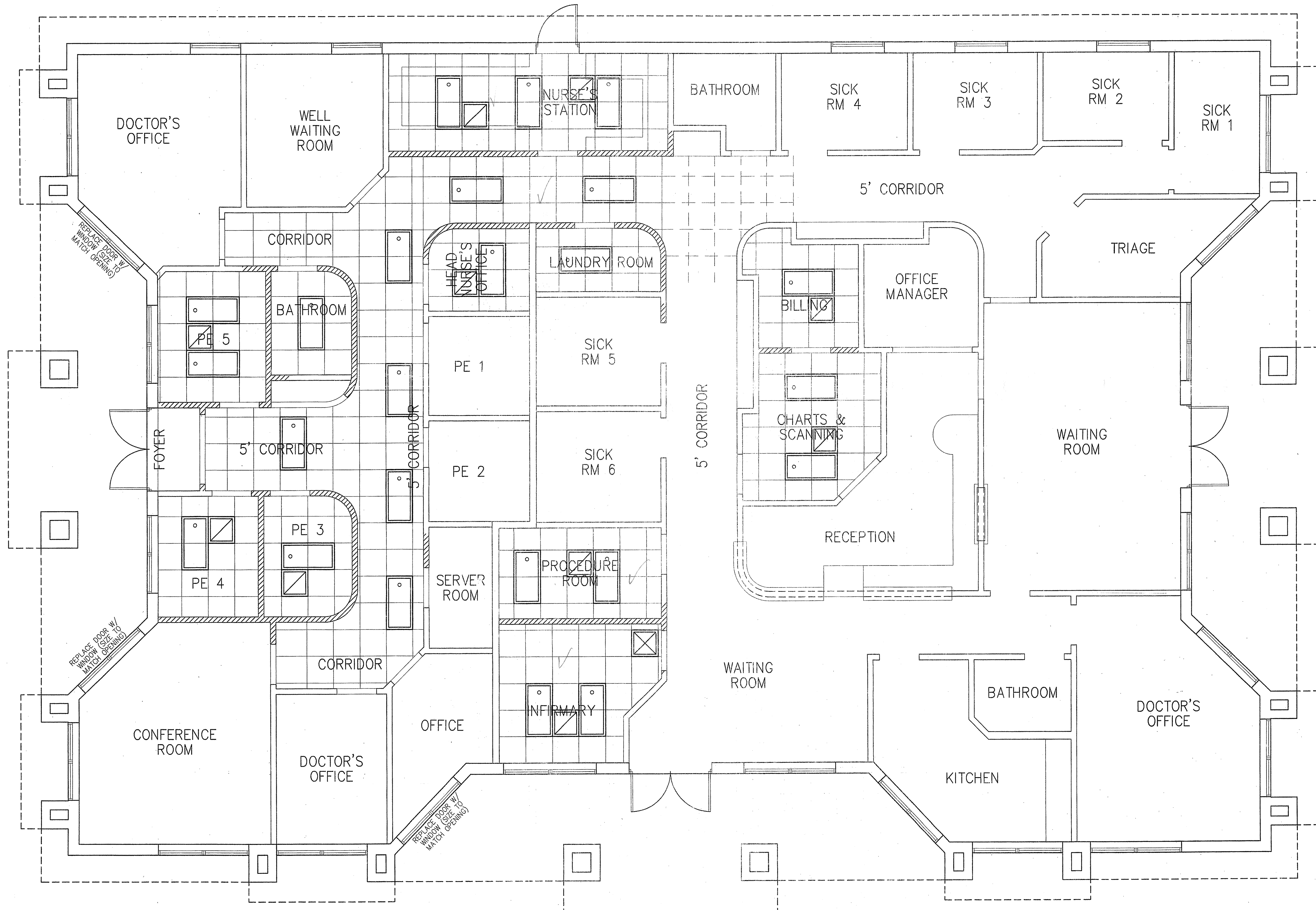
REFLECTIVE CEILING PLAN
