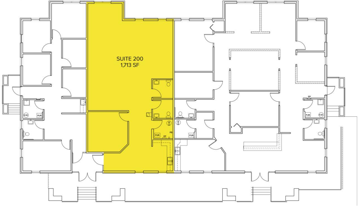
LOWER LEVEL AS-BUILT FLOOR PLAN 11,892 GROSS SQ.FT. 5,788 LOWER LEVEL SQ.FT. (1,263 - 4,540 SQ.FT. AVAILABLE)
