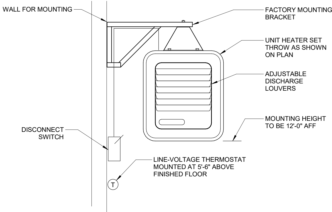
2 M-202 ELECTRIC UNIT HEATER DETAIL SCALE: NTS
