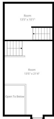
2nd Floor
