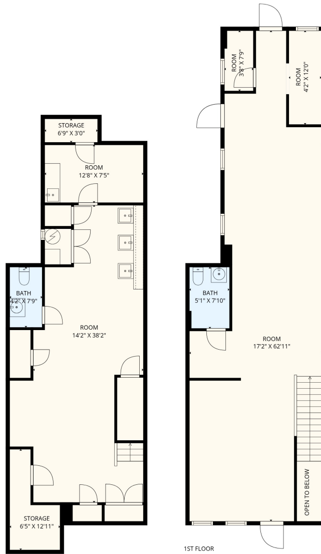
1ST FLOOR
