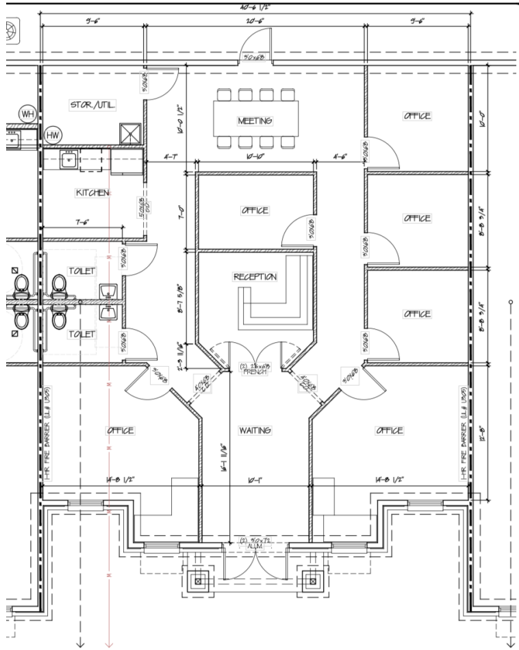
LEASE SPACE #1 BUILD-OUT 1/4" = 1'-0"
