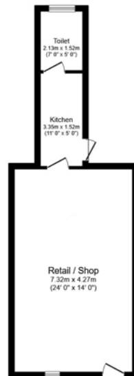
Floor Plan Floor area 39.9 sq.m. (429 sq.ft.)
