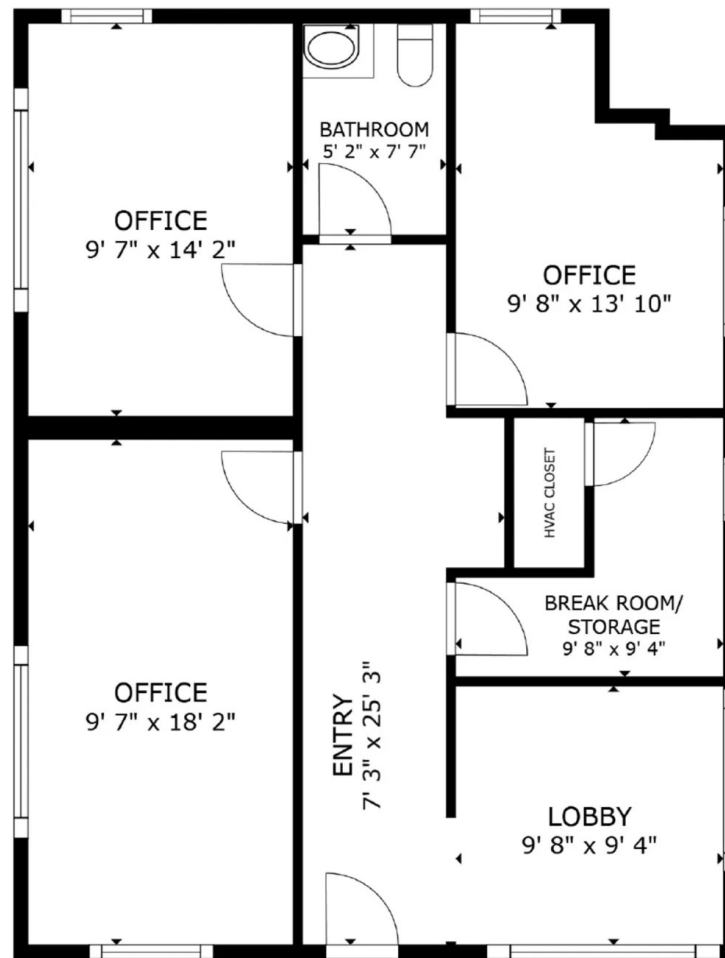
FLOOR PLAN
