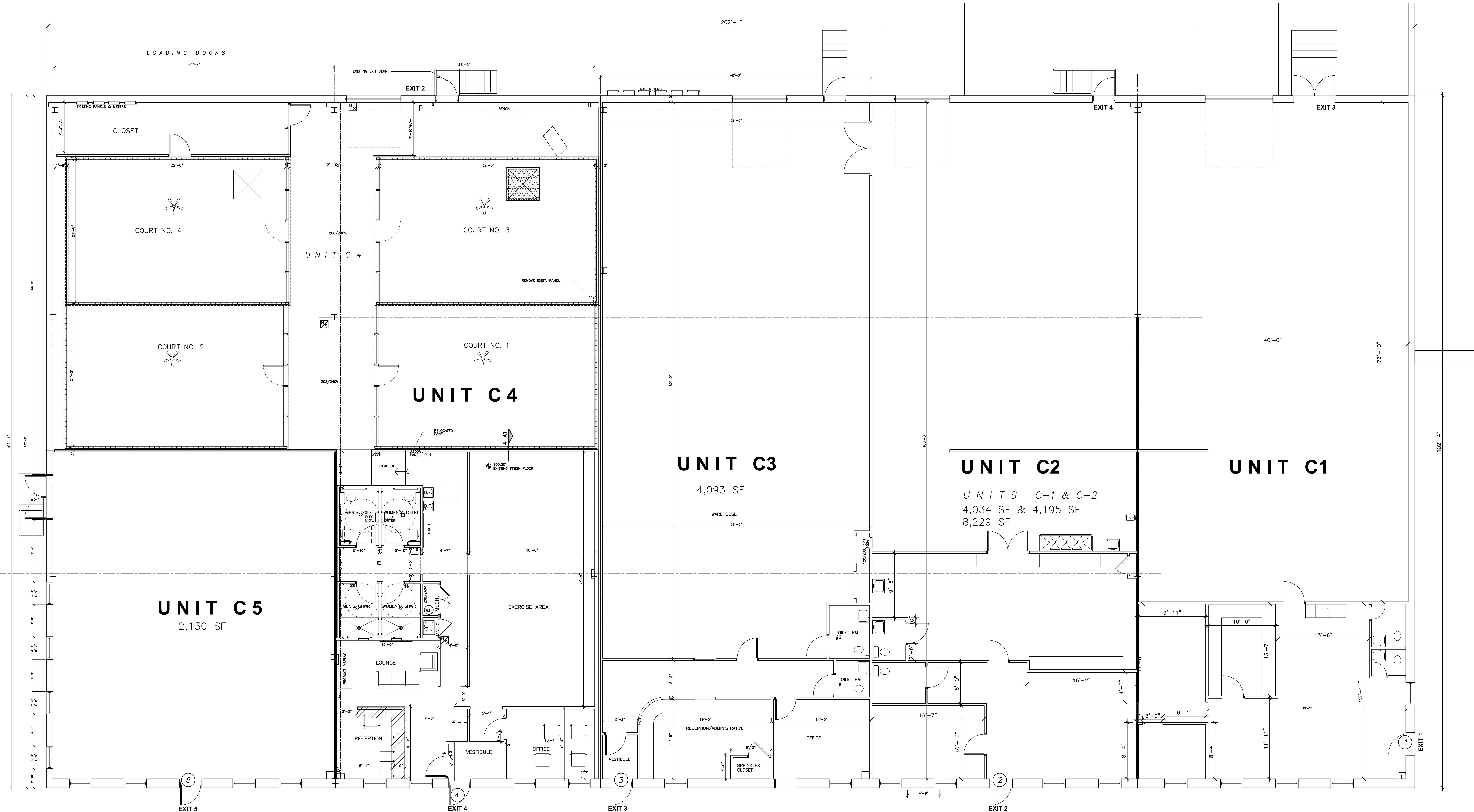
1 FIRST FLOOR PLAN 1/8" = 1'-0"
