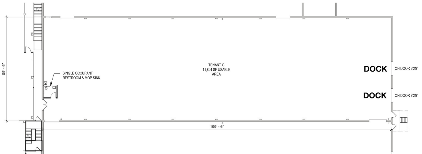
1 LOD1 Floor Plan 1" = 20'-0"
