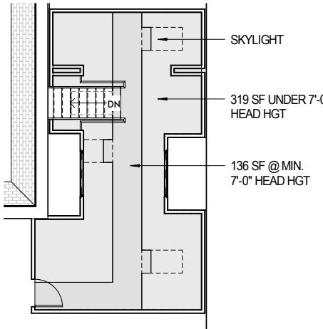
② Attic/loft Floor - Suite 2 1/8" = 1'-0"
