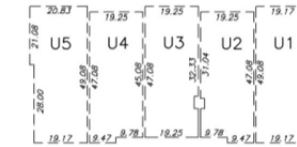
2nd Level of 2nd Floor Units, BLDG N UNIT DETAILS
