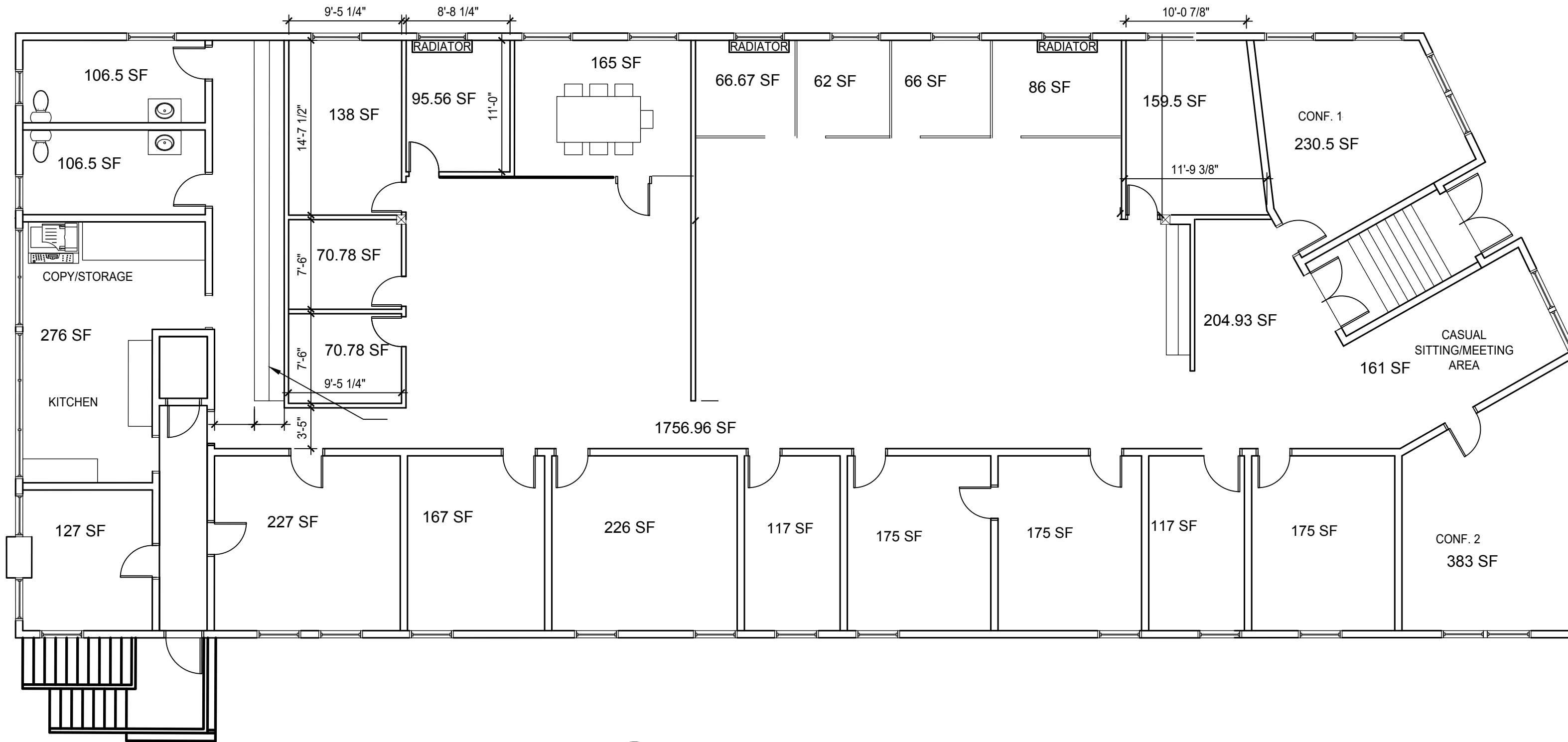
2 FLOOR PLAN SCALE: 1/8" = 1'-0" TRUE NORTH
