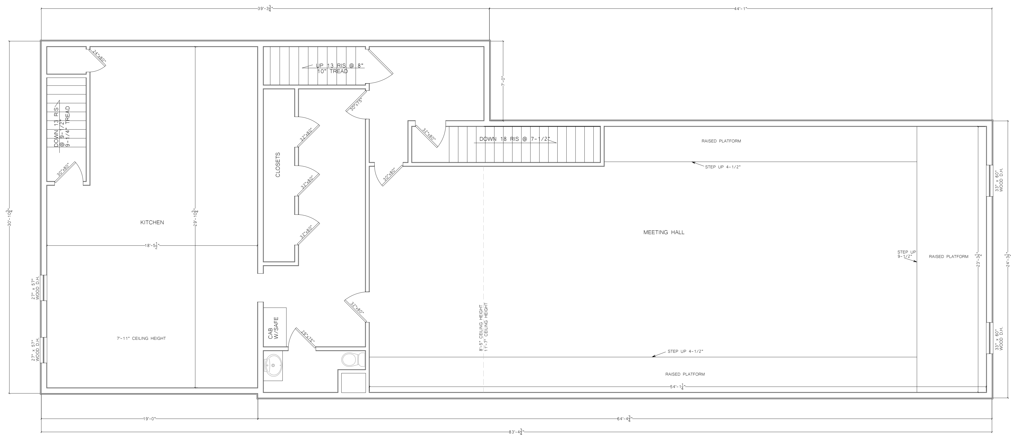
EXISTING SECOND FLOOR PLAN 1/4"=1'-0" 11/6/2017
