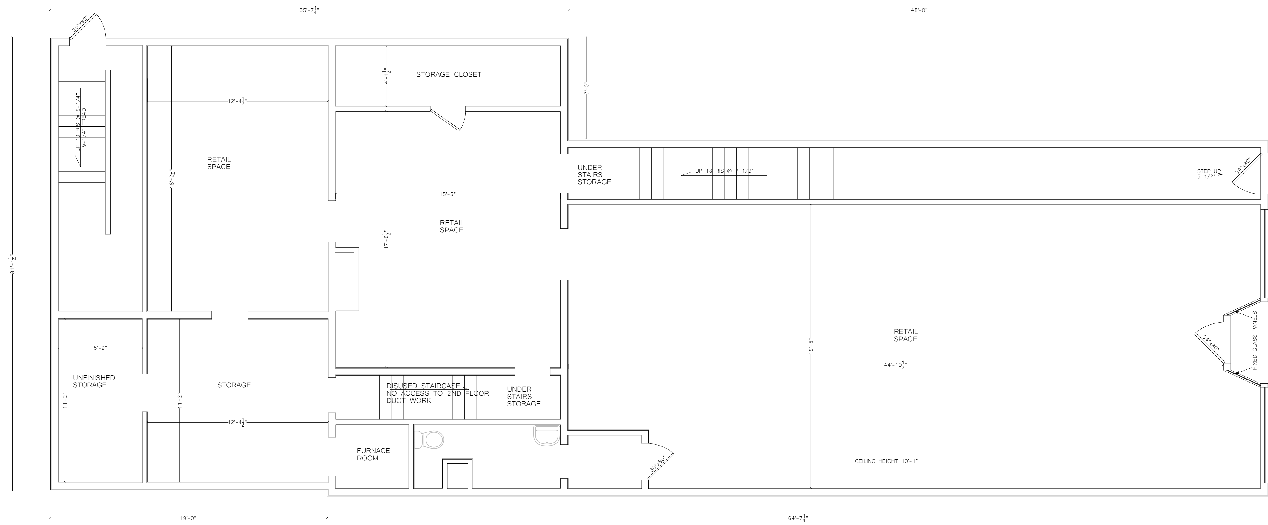
EXISTING FIRST FLOOR PLAN 1/4"=1'-0" 11/6/2017
