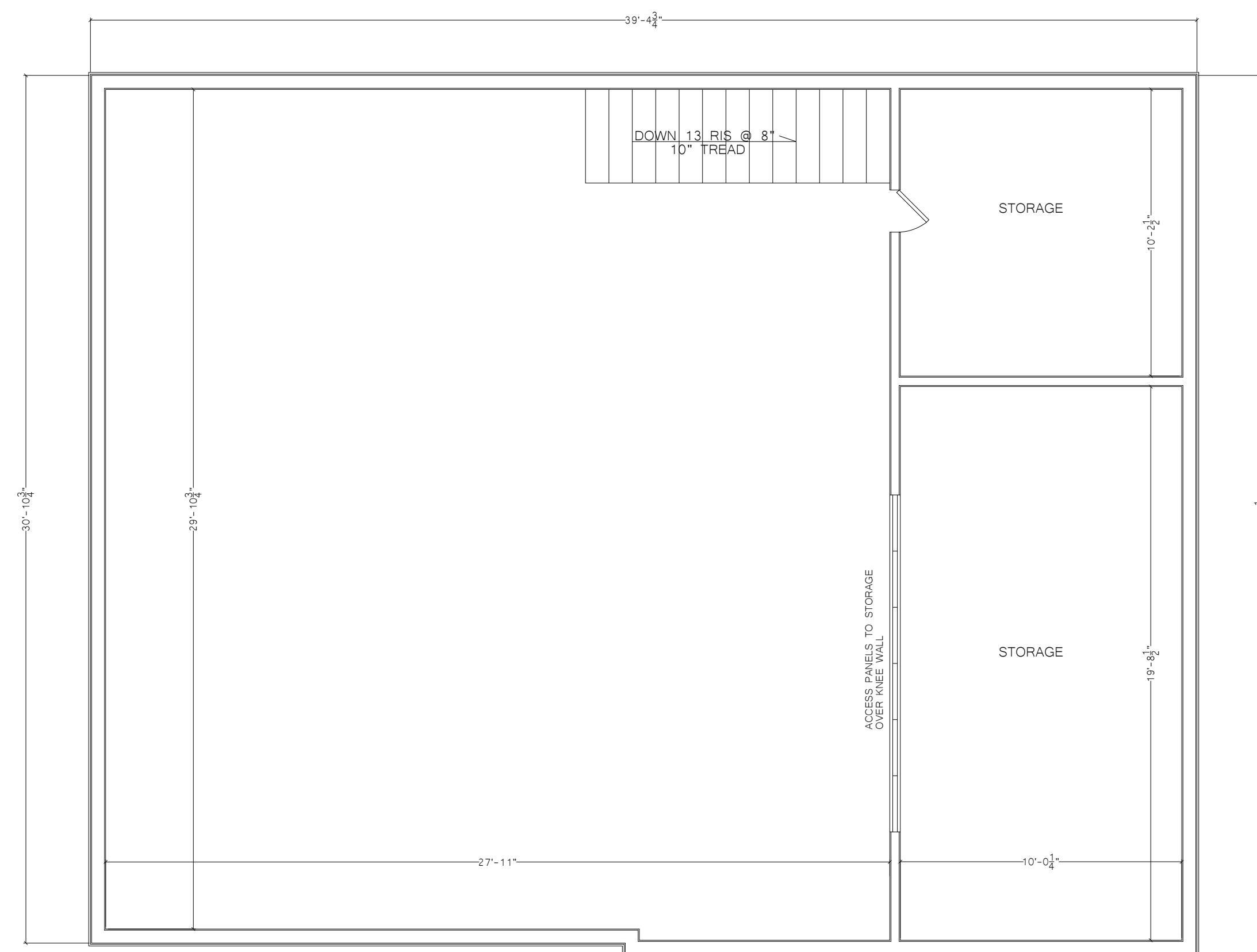
THIRD FLOOR PLAN 1/4"=1'-0" 11/6/2017
