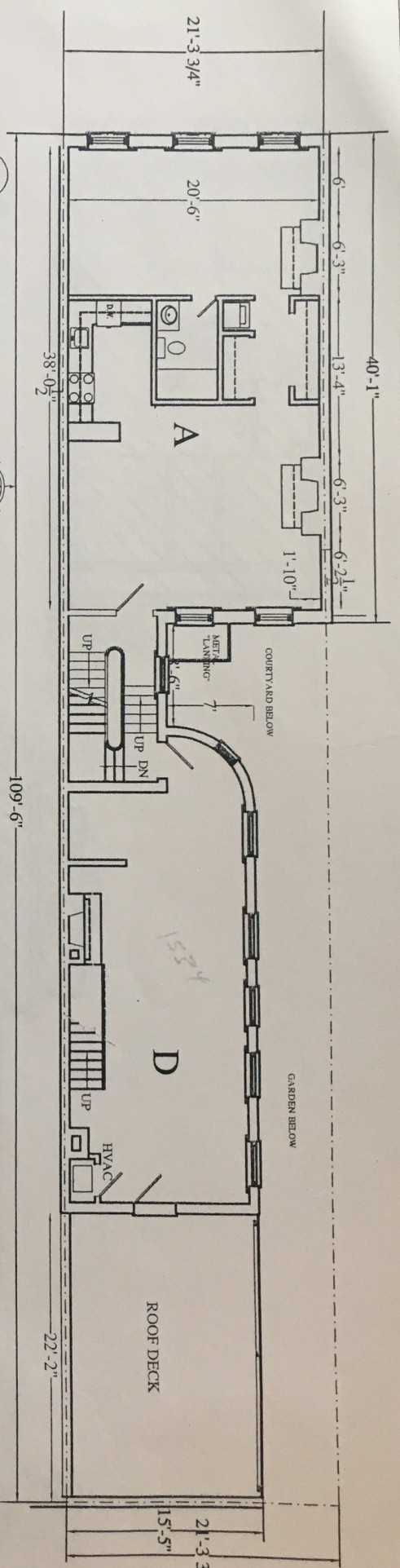
2 SECOND FLOOR PLAN A2 NOT TO SCALE
