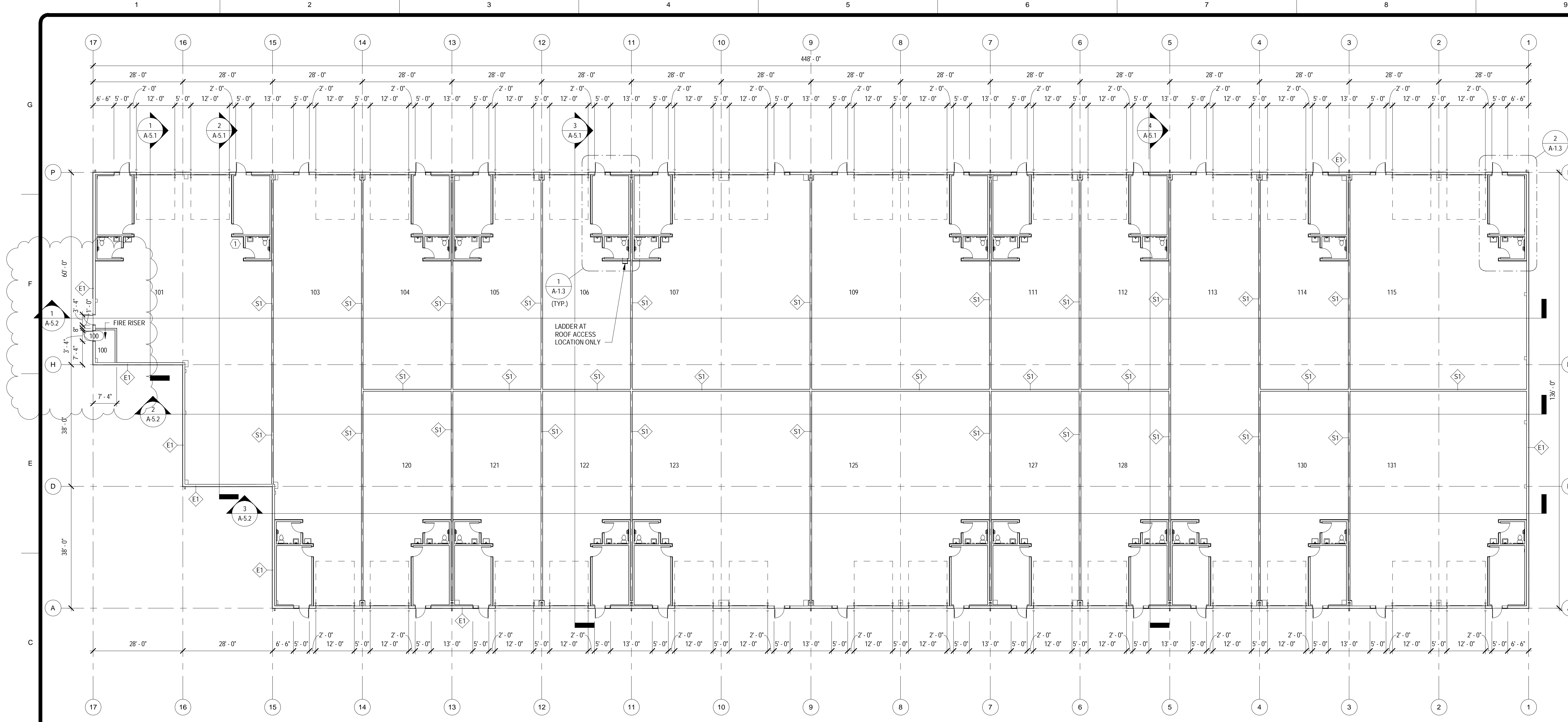
1 BUILDING A - FLOOR PLAN - 1ST FLOOR A-1.1 SCALE: 1/16" = 1'-0"
