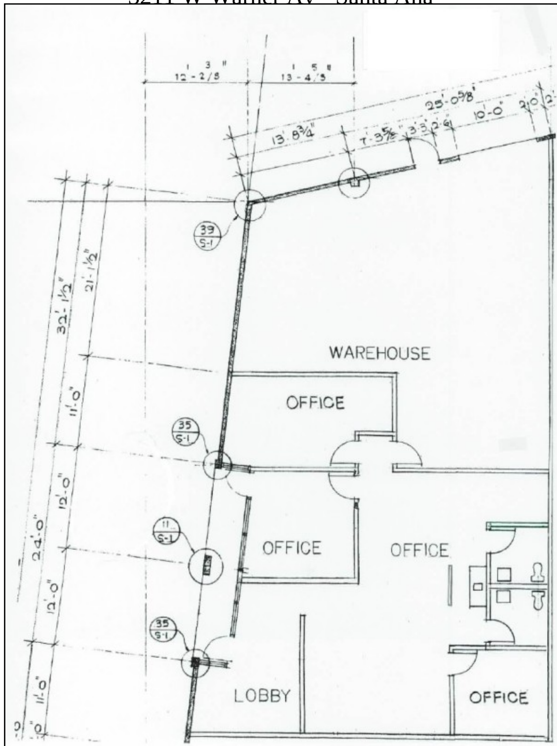
FLOOR PLAN
