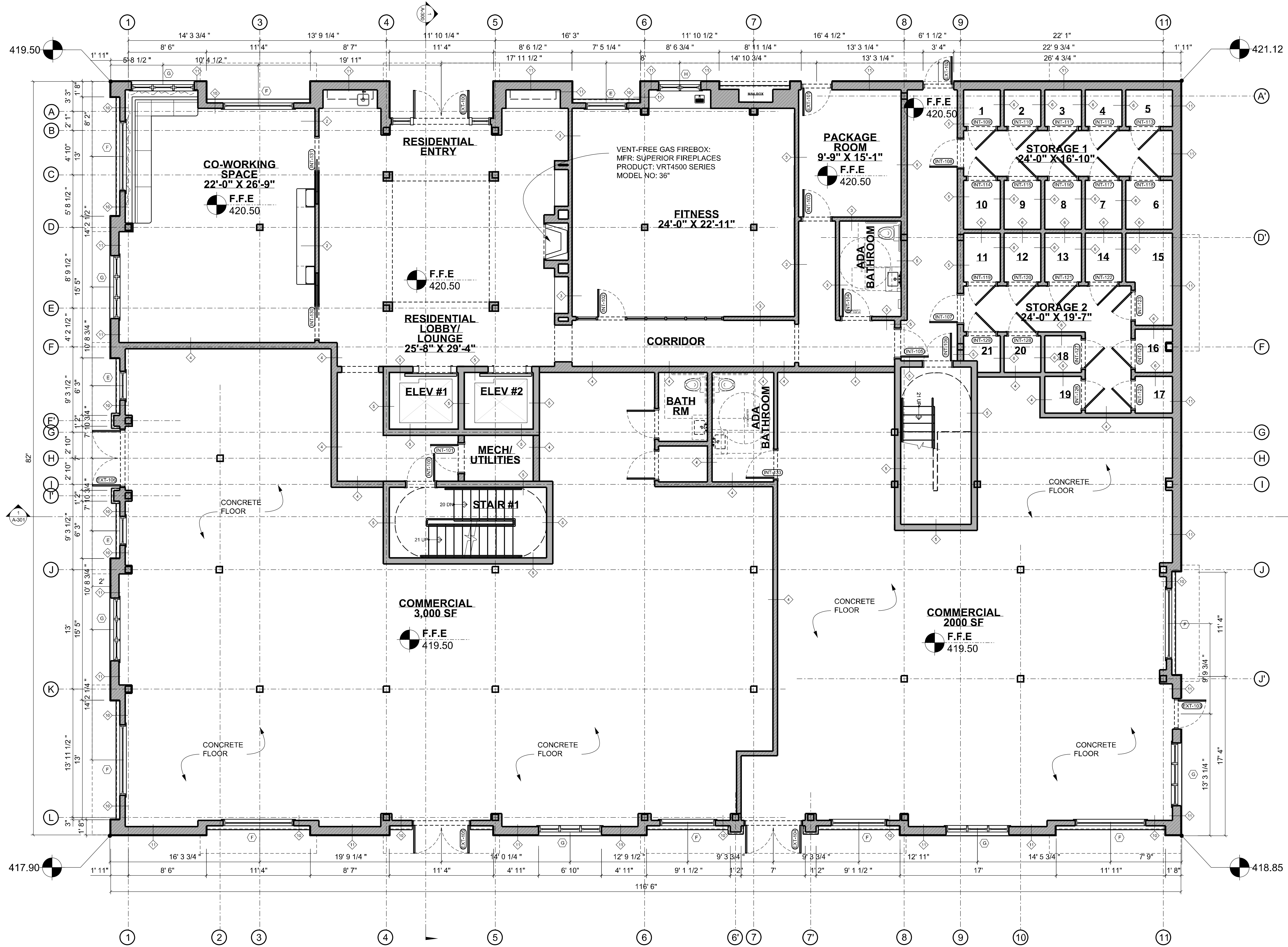
1/A-101 PROPOSED FIRST FLOOR PLAN 3/16" = 1'-0"
