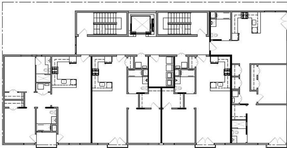
529-531 Mulberry Street Typical Floor Plan 2-4
