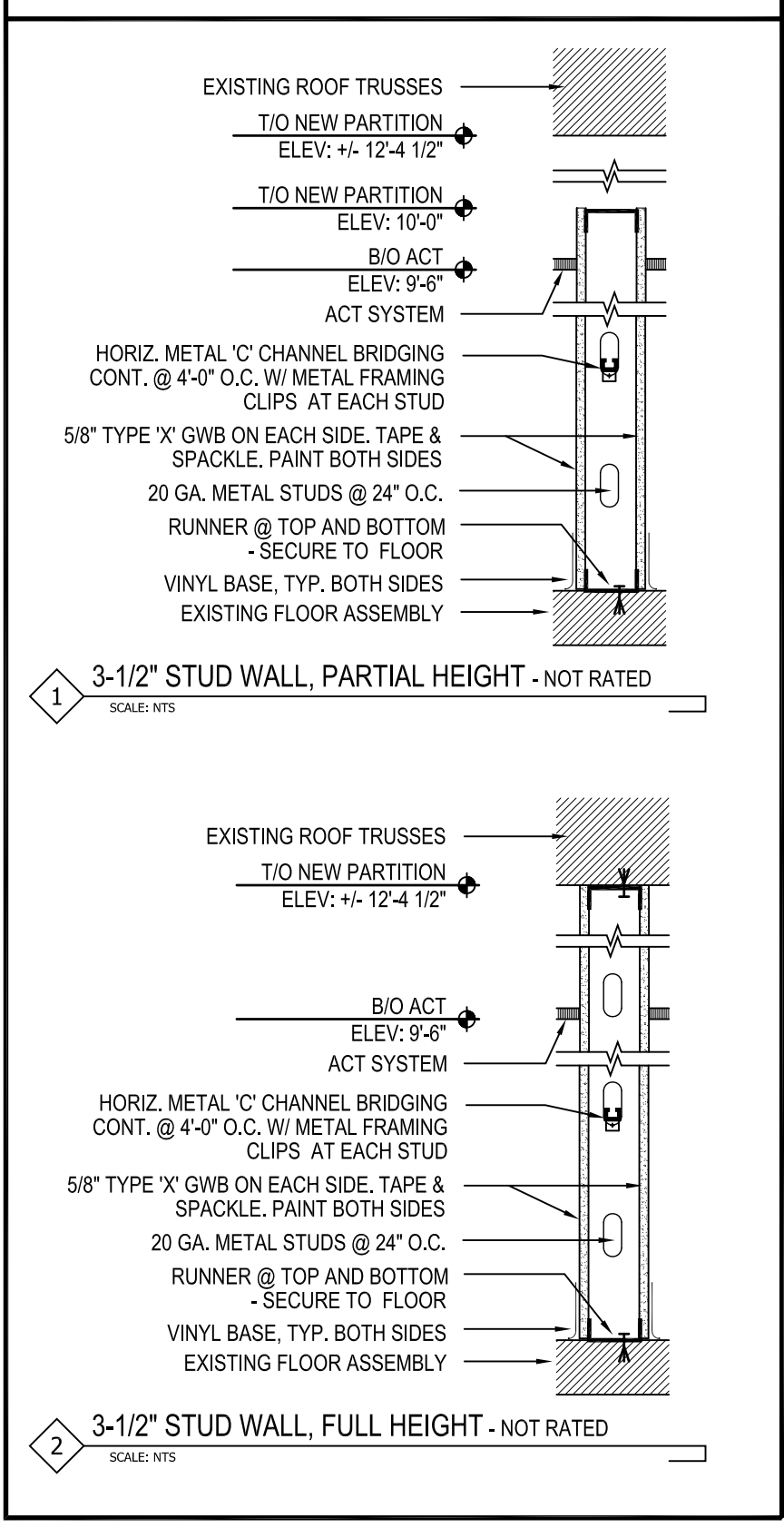
2 WALL TYPES A1.1 SCALE: NTS
