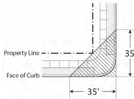
FIGURE 17.C.02.030-1: VISIBILITY TRIANGLE
