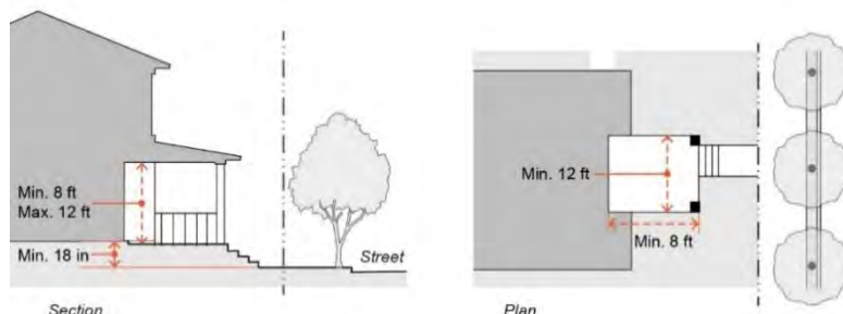
FIGURE 17.C.10.180-7: PORCH FRONTAGE
