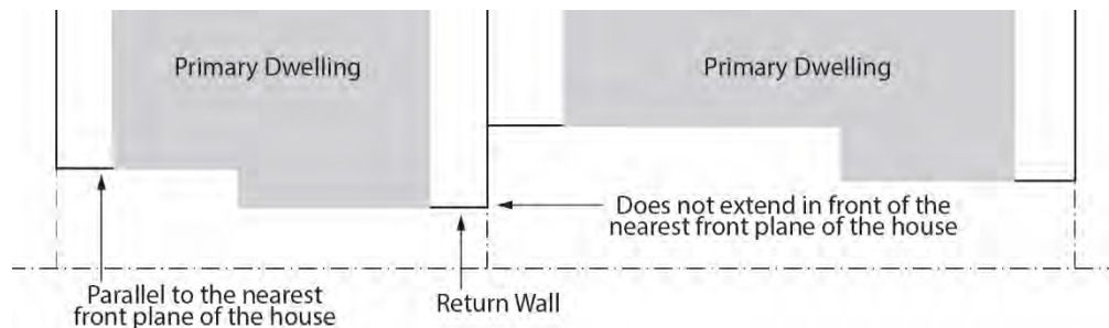
FIGURE 17.C.02.030-2: RETURN WALL
