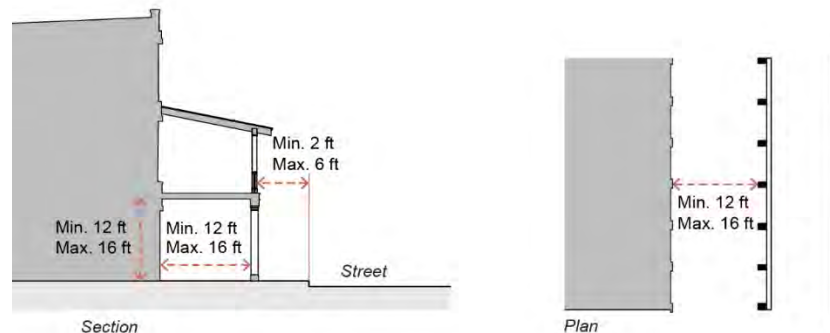
FIGURE 17.C.10.180-11: GALLERY FRONTAGE
