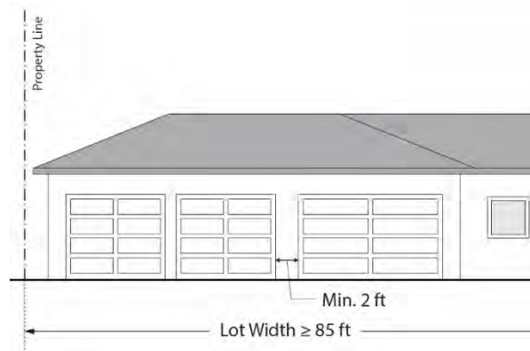
FIGURE 17.C.10.210-5: THREE-CAR GARAGES
