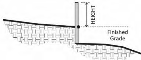
FIGURE 17.A.06.080-1: MEASURING HEIGHT OF FENCES AND WALLS
