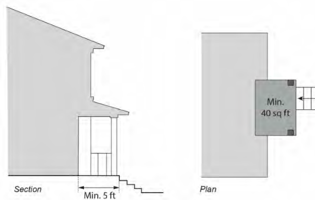
Figure 17.C.10.210-1: Entrance Protection
