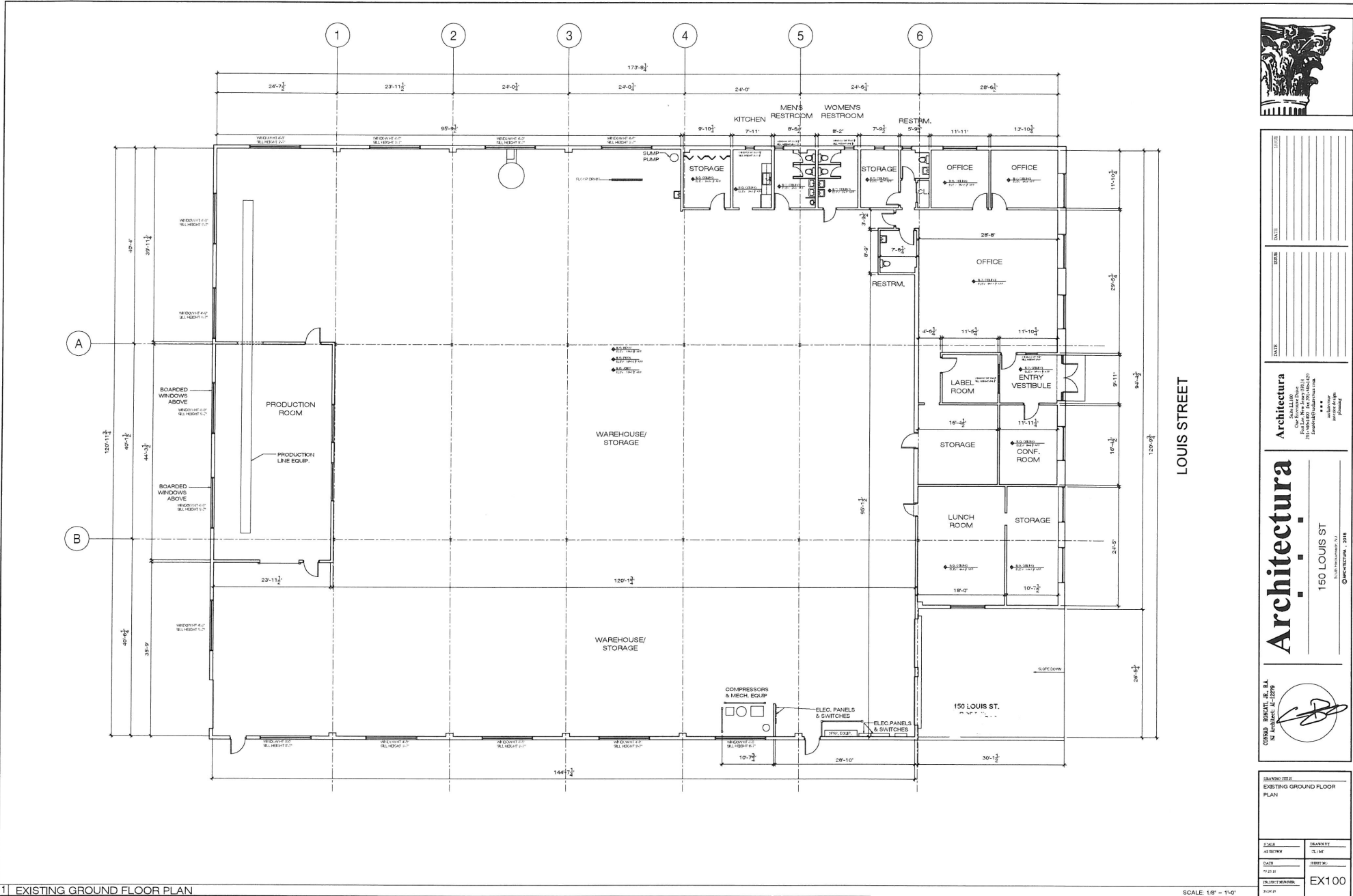
1 | EXISTING GROUND FLOOR PLAN
