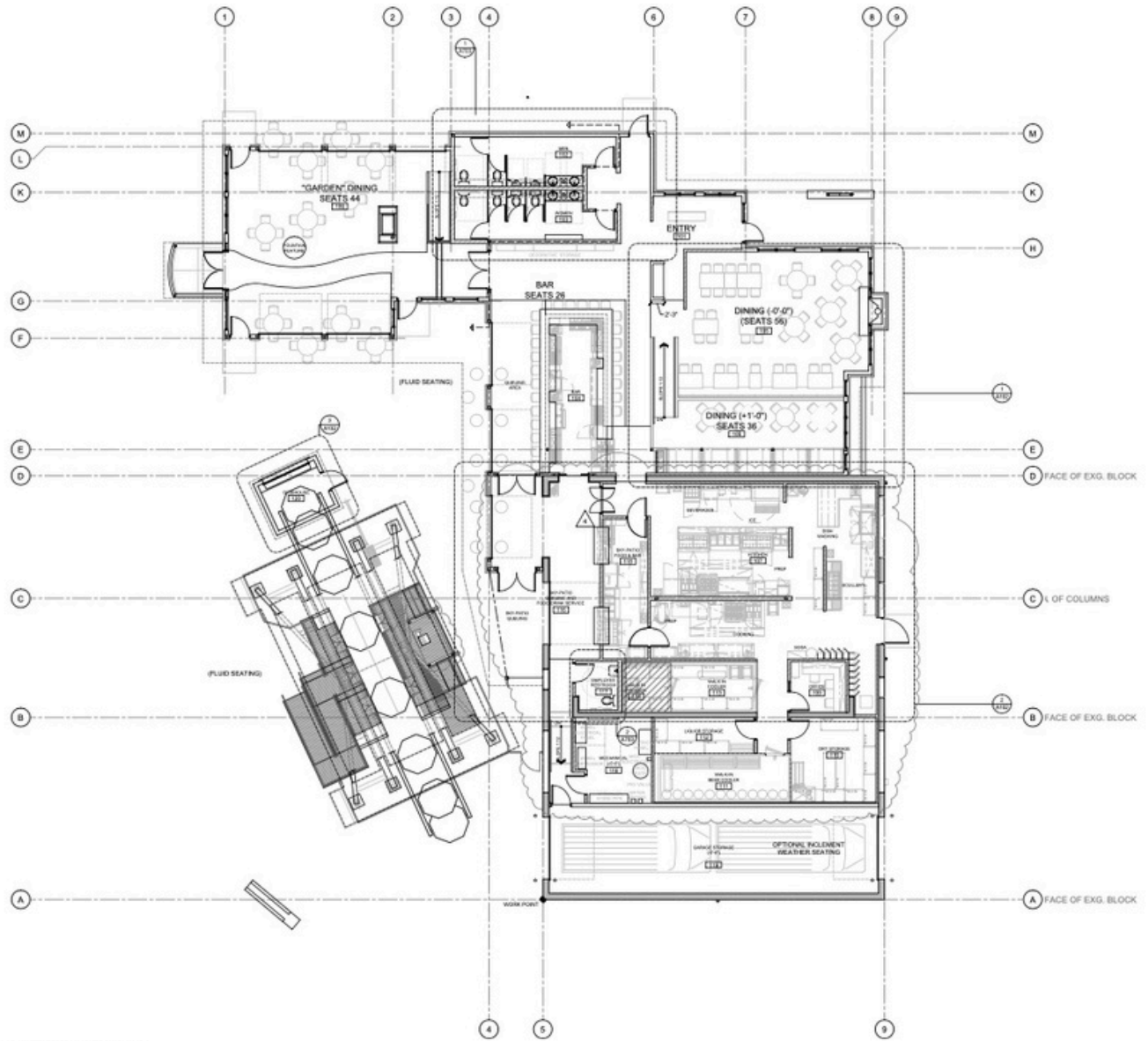
FURNITURE & FIXTURE PLAN
