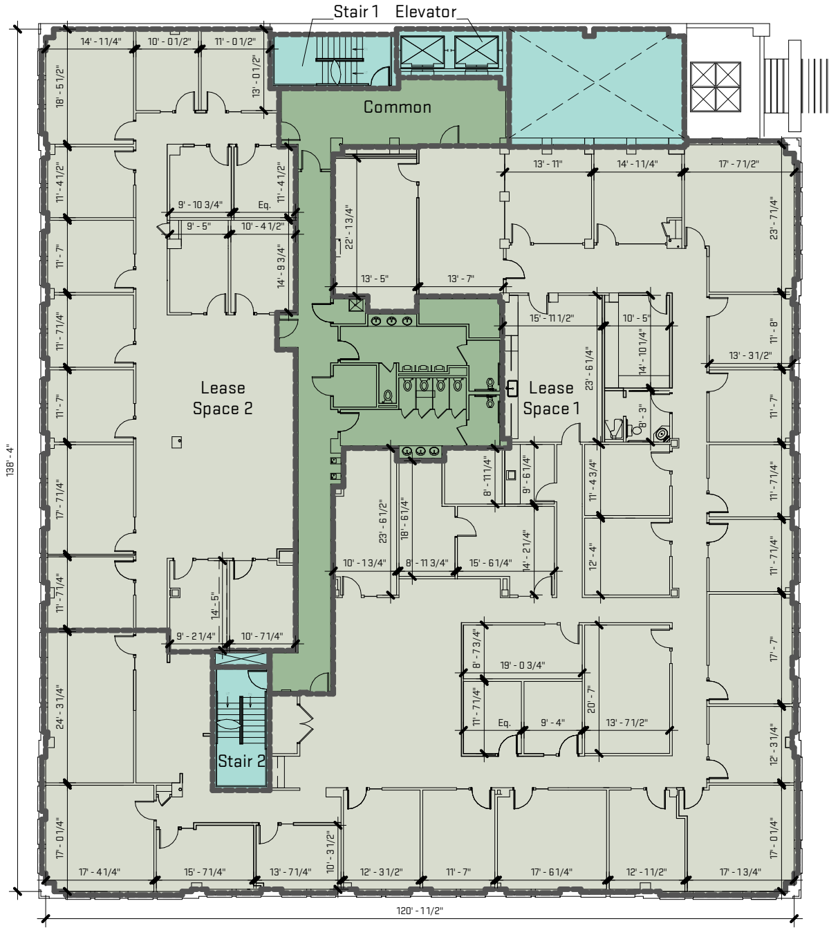
Level 2 - Floor Plan 3/64" = 1'-0" 16' 32' 48'
