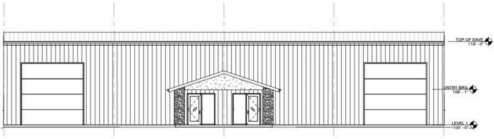
9 FRONT ELEVATION 1/8" = 1'-0"
