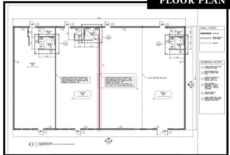
FLOOR PLAN
