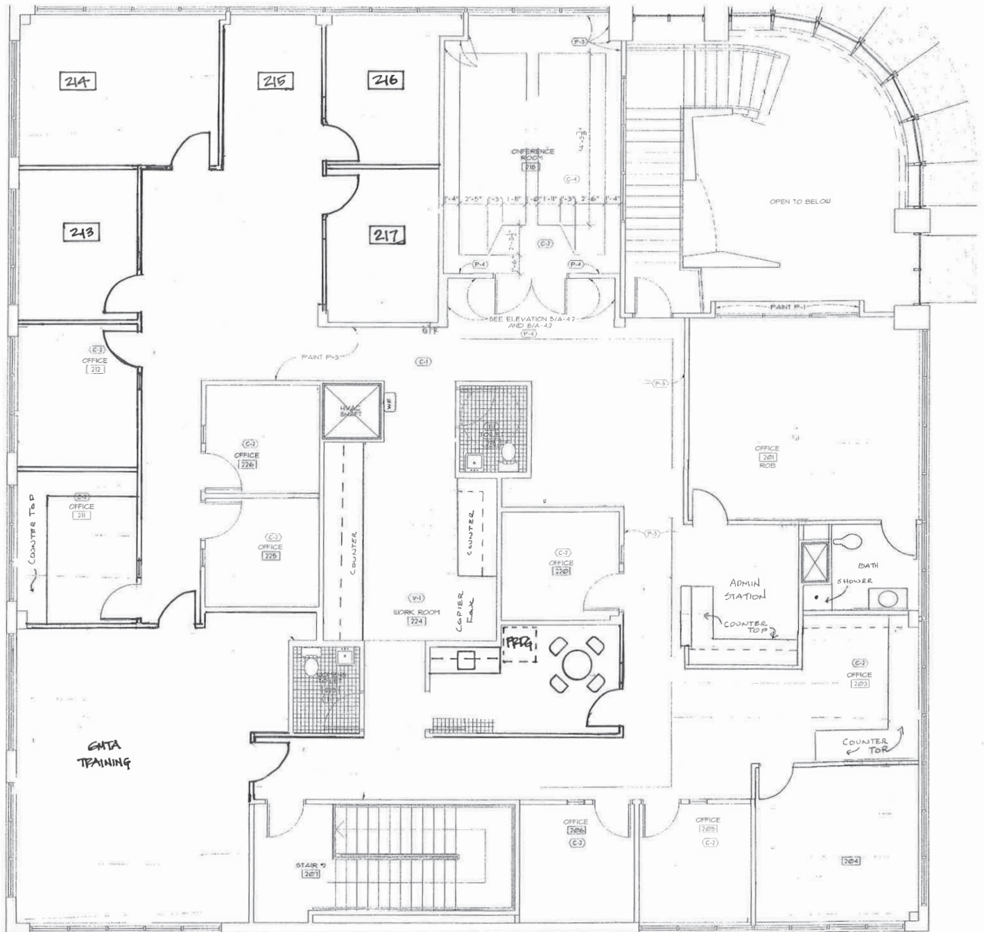
1 SECOND FLOOR FINISH PLAN A-62 1/4"=1'-0"
