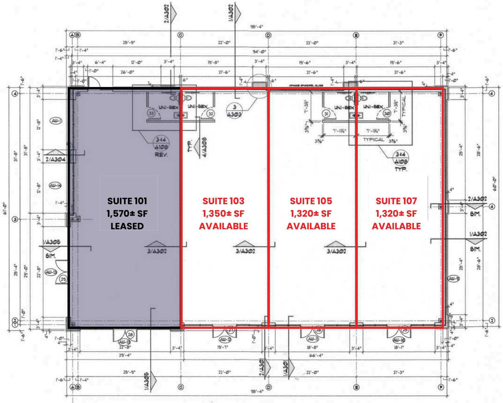
OVERALL FLOOR PLAN BUILDING "B" 1/8" = 1' - 0"
