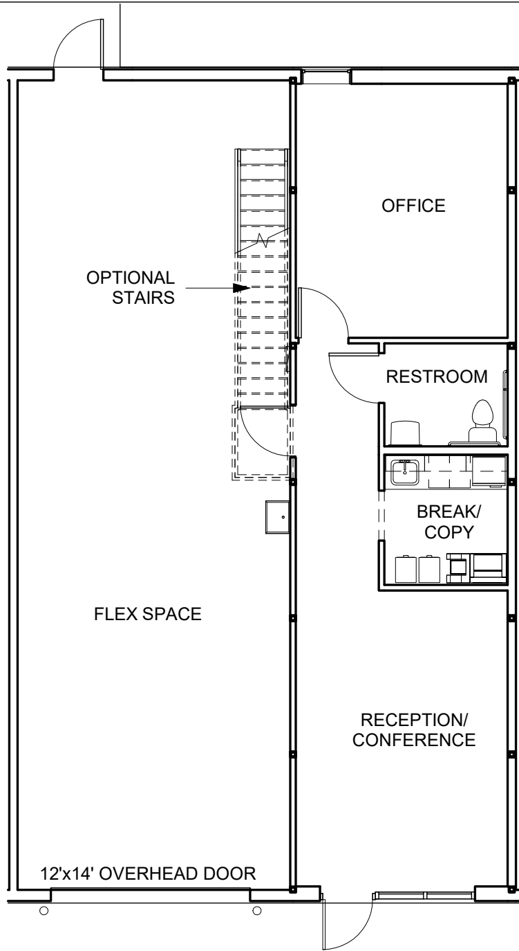
① Marketing Main Floor Plan - Suite 110A 1/8" = 1'-0"
