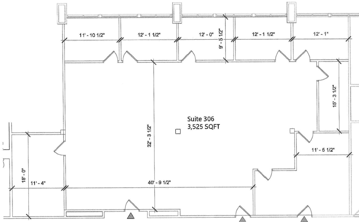
① SUITE 306 1/8" = 1'-0"
