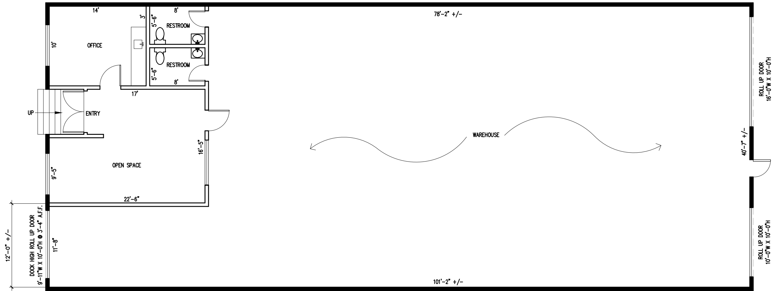
1 FLOORPLAN (4,105 +/- SQ. FT.) 1/8"=1'-0"
