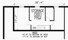
MEZZANINE LEVEL PLAN (±775 SF) 1/16" = 1'-0"
