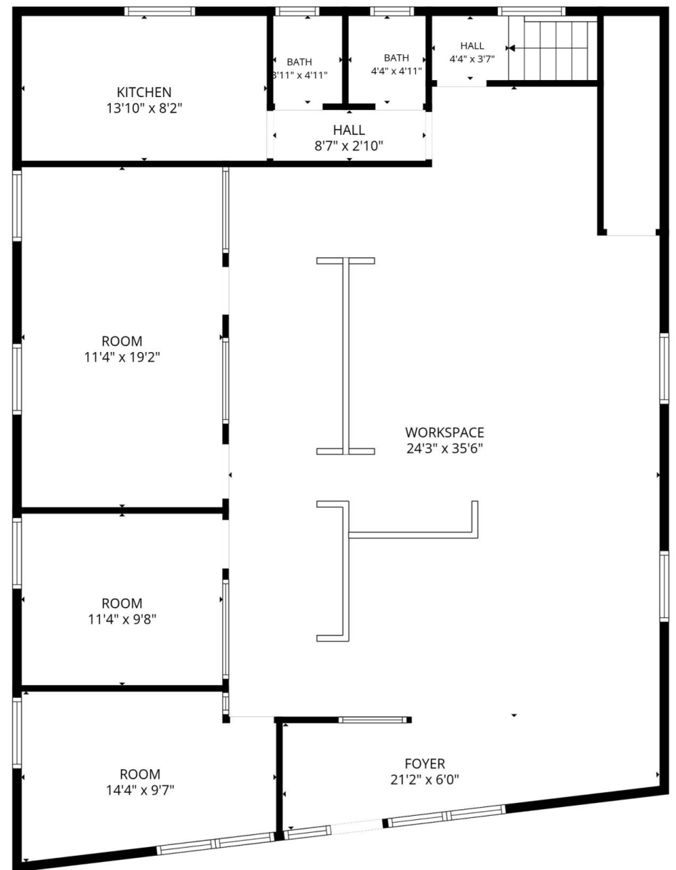
2nd floor
